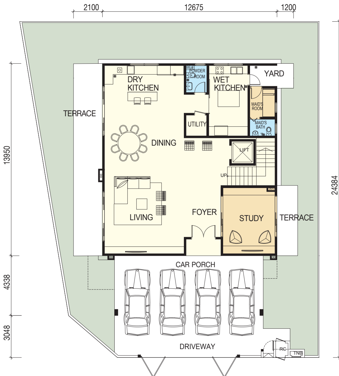
GROUND FLOOR
