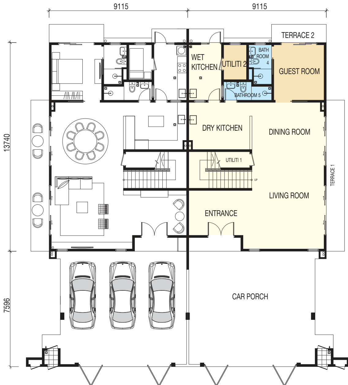
GROUND FLOOR
